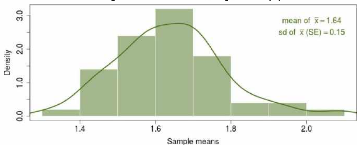
Distribution of means of 50 random samples, each consisting of 150 observations from a right skewed population
